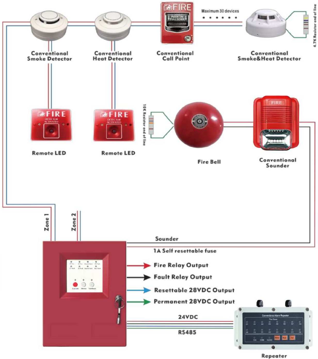
2 Zones Conventional Fire Alarm Control Panel
